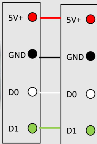
Card Reader
