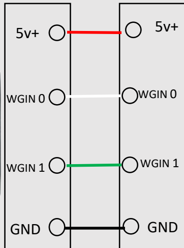
Card Reader
