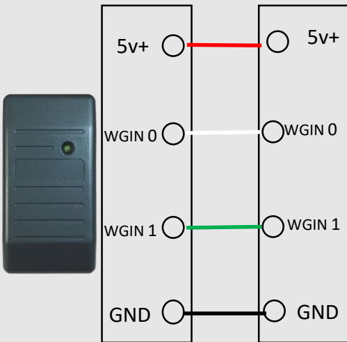
Card Reader
