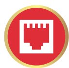
TCP/IP
